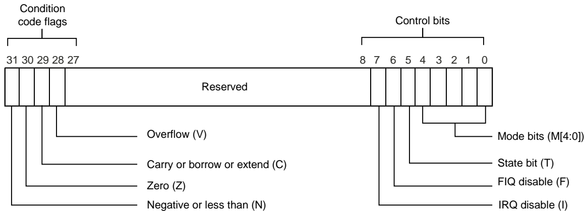
Figure 2-6 Program status register format
